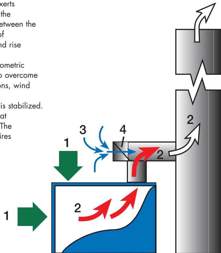
Illustration A Gas Installation
